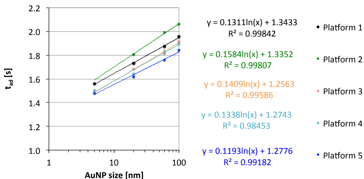
Figure S1: Obtained correlations of t_{ad} and AuNP size with different graphite platforms used as sample carrier.
