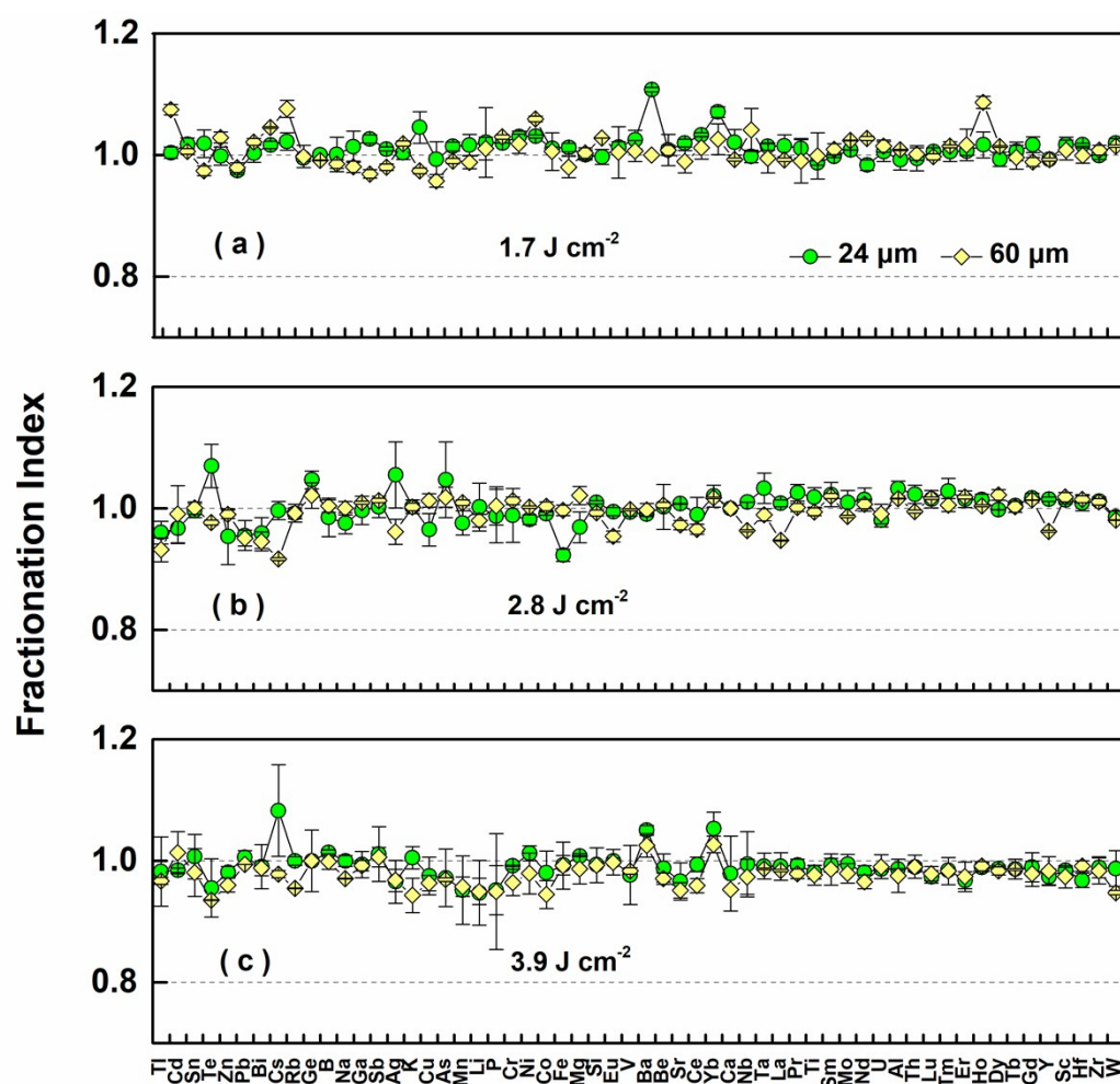
SFig 1. The Ca-normalized fractionation indices (FIs) by femtosecond laser ablation of NIST 610 at different fluences. (a): 1.7 \text{ J cm}^{-2} ; (b): 2.8 \text{ J cm}^{-2} ; (c): 3.9 \text{ J cm}^{-2} . Error bars represent the standard deviation (1 s) from three measurements.
