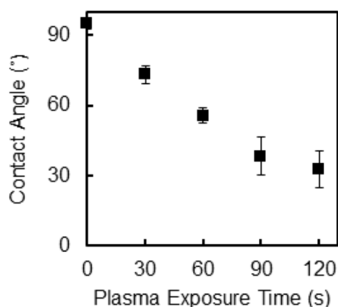
Fig. S1 The critical advancing contact angle of PBS on PDMS as a function of oxygen plasma exposure time. Error bars represent standard error.
