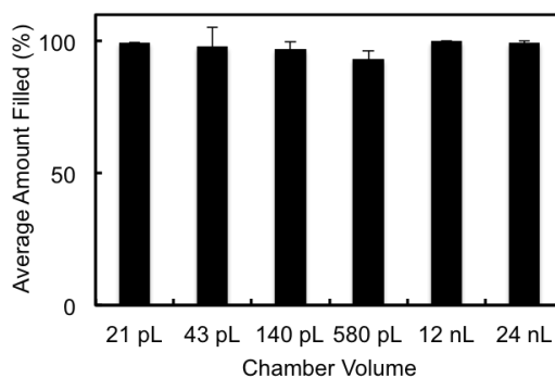
Fig. S2 Accuracy of filling as a function of chamber size.
