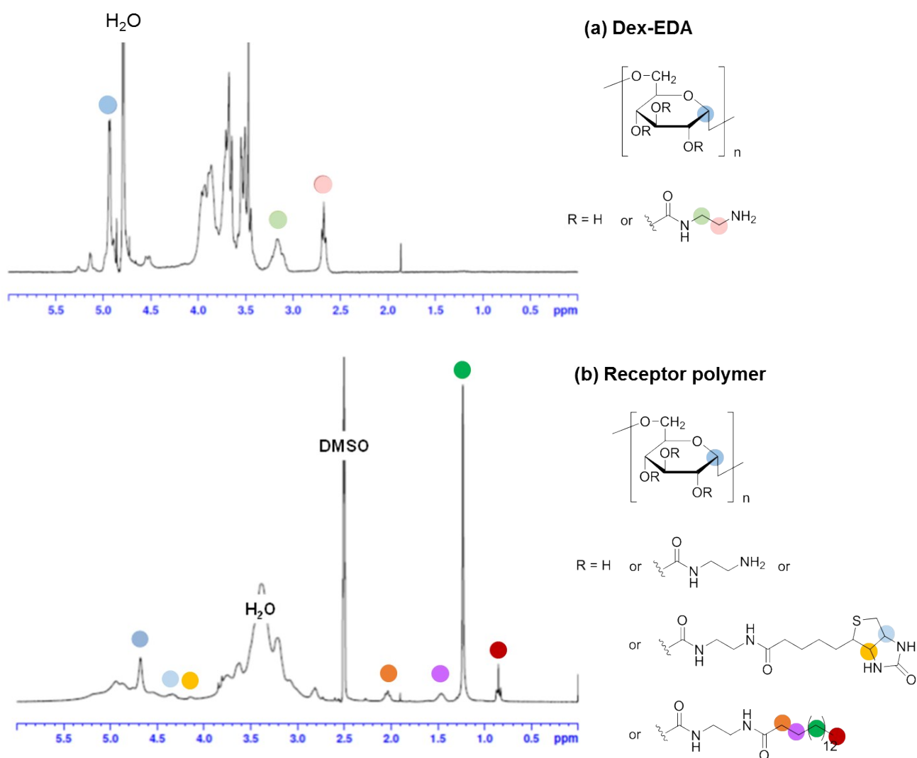
Fig. S1. ^1\text{H} NMR spectra (300 MHz, r.t.) of (a) Dex-EDA (in \text{D}_2\text{O} ) and (b) receptor polymer (in DMSO).
