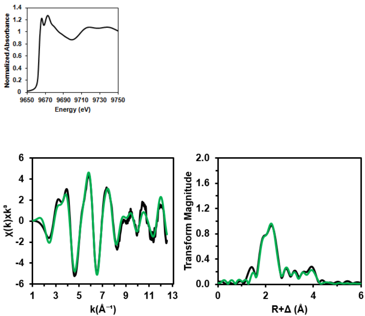
Supplemental Figure 9. XAS of Zn(II)-SlyD. (Top) Zn(II) near-edge spectrum of Zn(II)-SlyD. SlyD was loaded with 0.7 equivalents of zinc. (Bottom) k^3 weighted Zn(II) EXAFS data (left) and Fourier transform data (right) of Zn(II)-SlyD (black). The best fit model (green) corresponds to a S_2/His_2 coordination environment.
