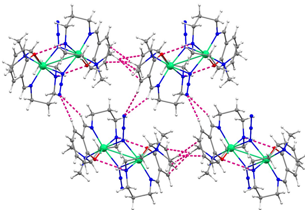
Fig. S2. Packing diagram of 3 showing different noncovalent interactions.
