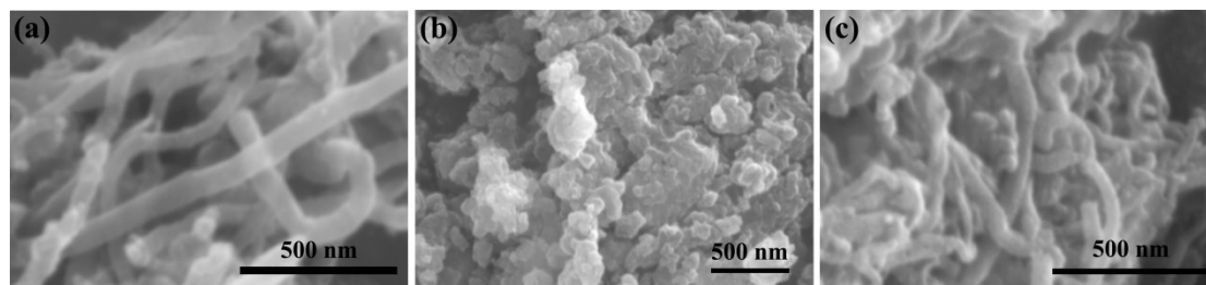
Fig. S2 SEM images of MWNTs, Fe 3 O 4 and Fe 3 O 4 @MWNTs after cycling.
