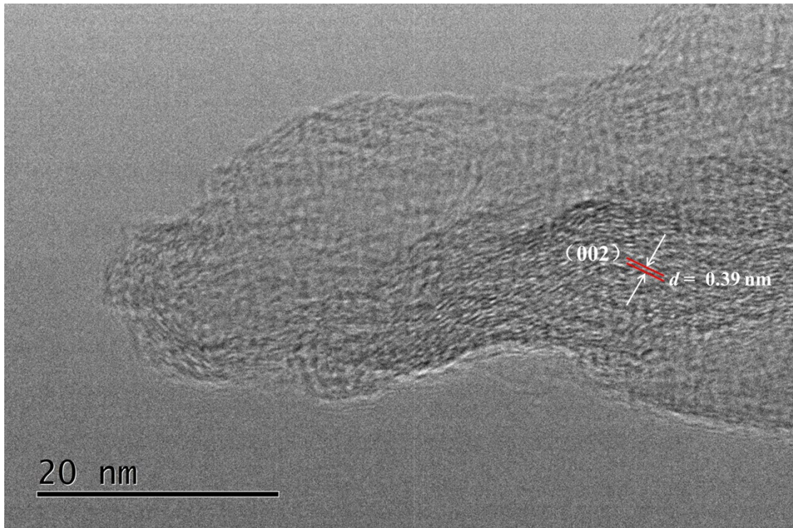
Fig. S1 HRTEM image of the resulting N-GANM.
