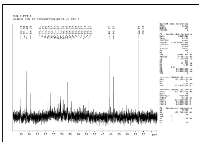
Figure S2. 13 C- NMR spectrum of Phosphorylated chitin (P-CTN).
