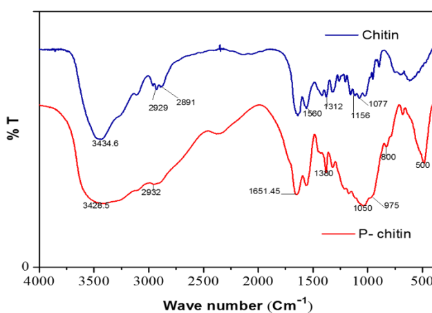
Figure S1. FTIR spectra of chitin (CTN) and Phosphorylated chitin (PCT)
