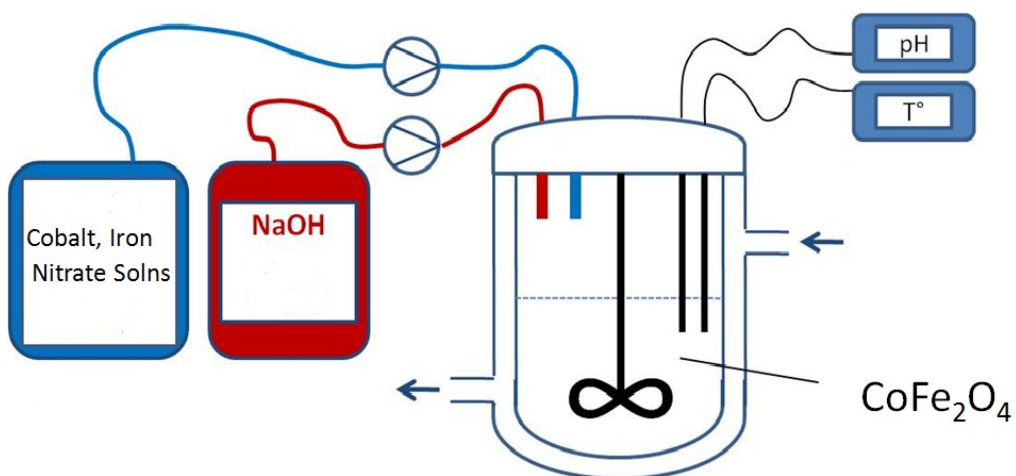
Figure S1: Schematic of the reactor
