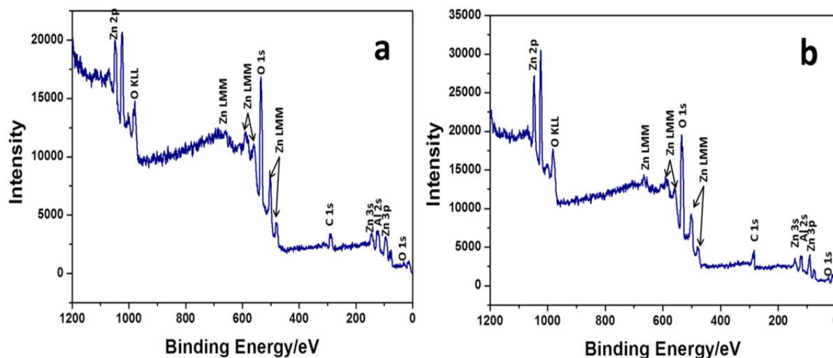
Figure S1. XPS survey spectra of (a) sample A and (b) sample E
