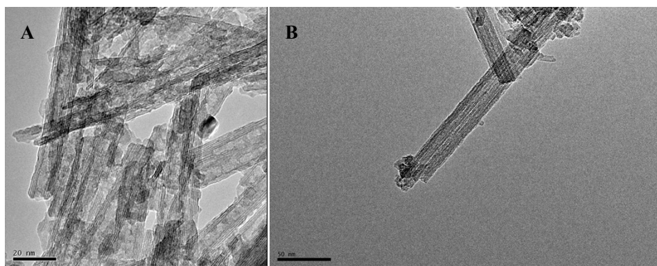
Fig. S1 TEM images of Rh/B-TNTs-Hydrothermal-5% (A) and Rh/B-TNTs-Impregnation-5% (B).
