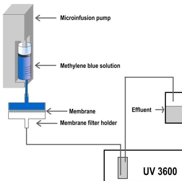
Fig. S1 Apparatus for degradation of methylene blue with AgNPs-immobilized polypropylene microfiltration membranes in a flow-through mode.
