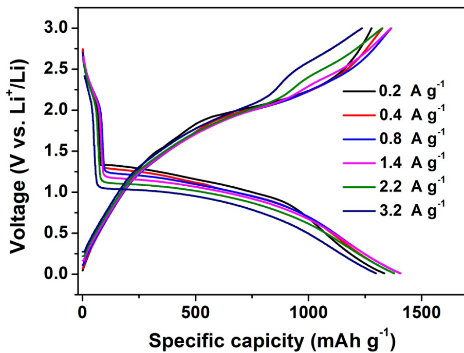
Fig. S3 Galvanostatic curves of hollow \text{Co}_3\text{O}_4 cube at different rates.
