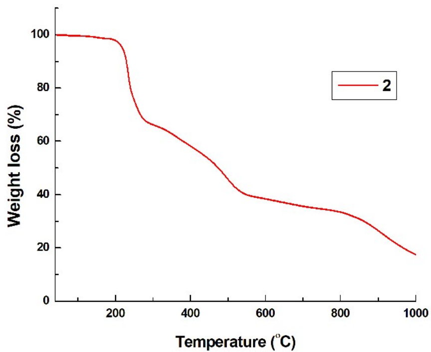
Fig. S2 TGA curve for 2.
