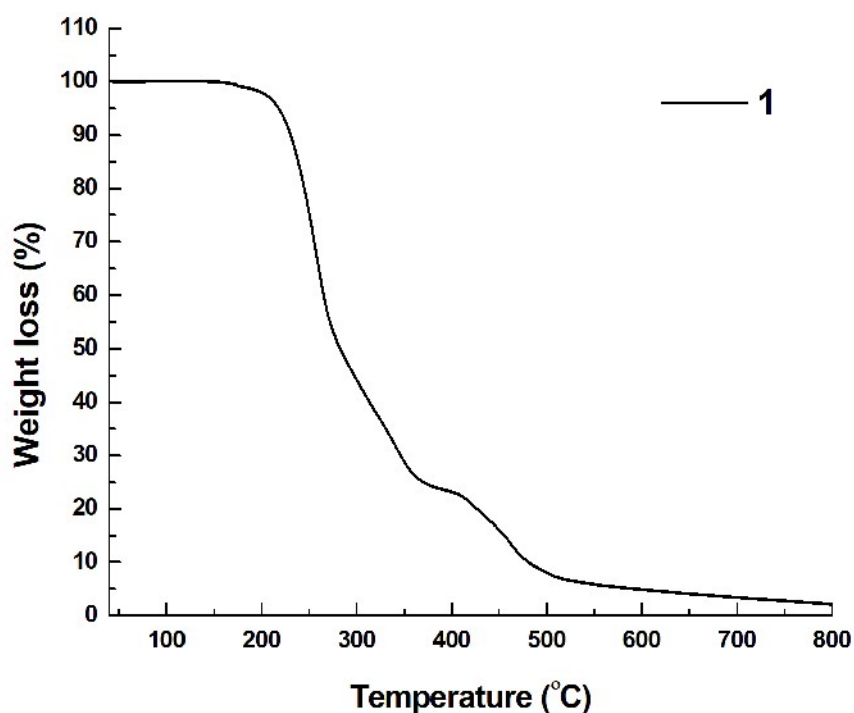
Fig. S1 TGA curve for 1.
