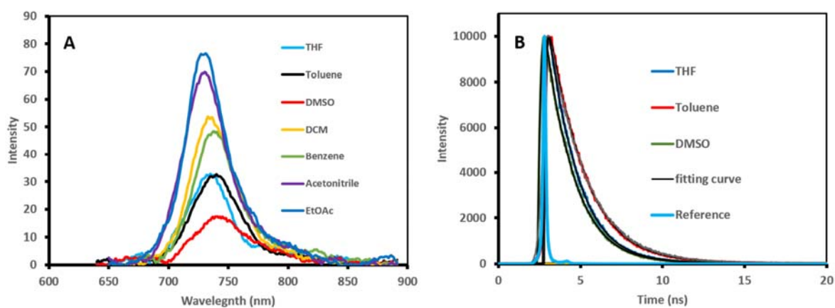
Figure S1. Fluorescence spectra of 1 (A) in different solvents-and (B) fluorescence decay curves of 1 in DMSO, THF and toluene.
