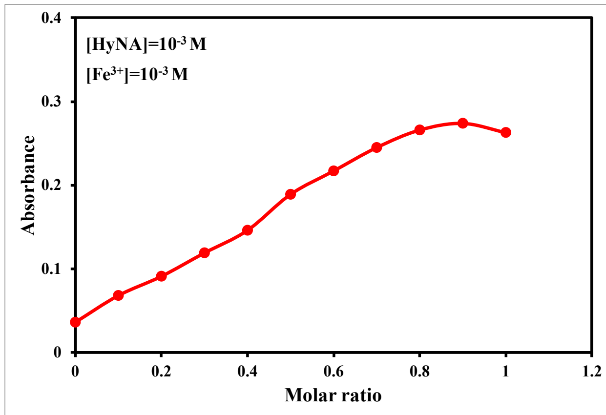
S-1: Molar ratio between Fe 3+ and HyNA reagent.
