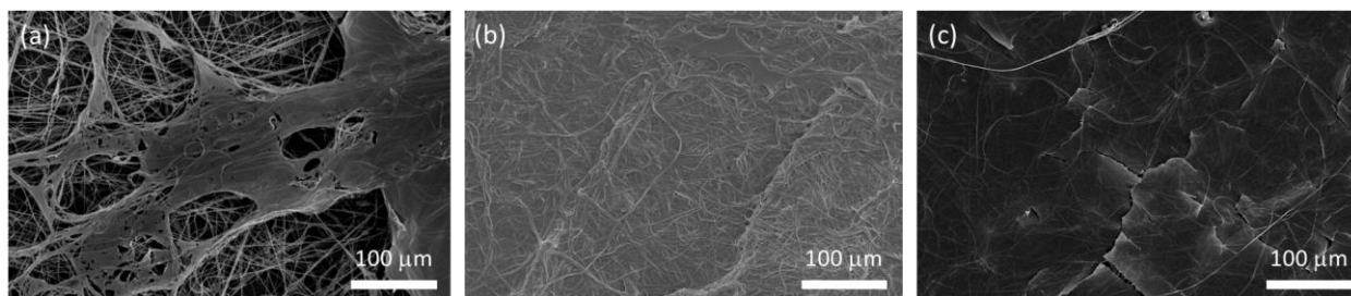
Figure S1. SEM images of PMMA-GO nanofibers using distinct adsorption times: (a) 30 min, (b) 1h and (c) 2h.
