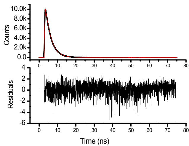
Figure S3: Fluorescence decay curve for complex 5 in DMSO
