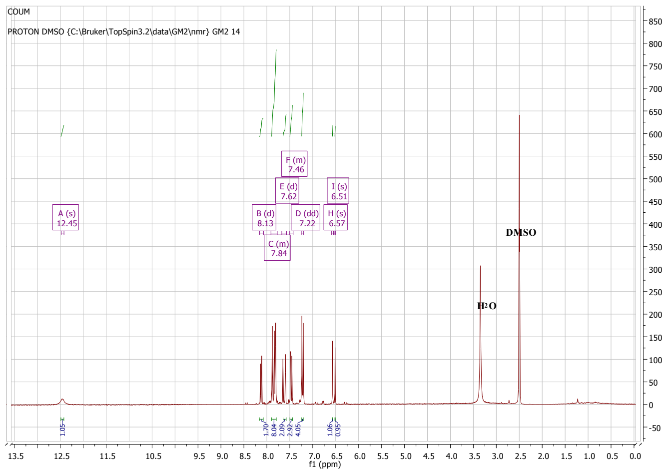
Figure S1: 1 H NMR spectra of 6
