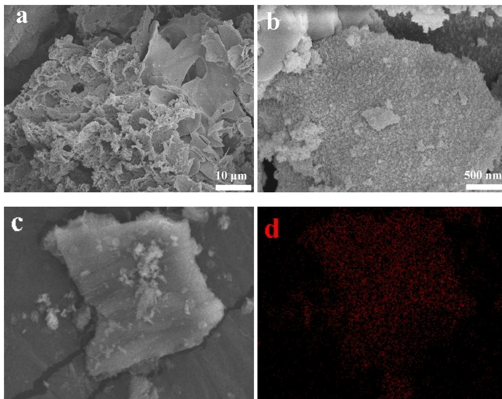
Fig. S2. (a and b) SEM images, SEM image (c) and the corresponding EDS mapping data for Cr (d) of MCRCS s obtained after four cycles of the photoreduction of Cr(VI)
