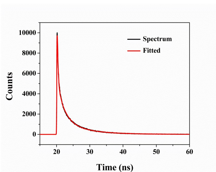
Fig. S2. Time-resolved fluorescence decay of N-CDs
