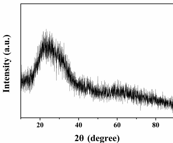
Fig. S1. The XRD pattern of N-CDs
