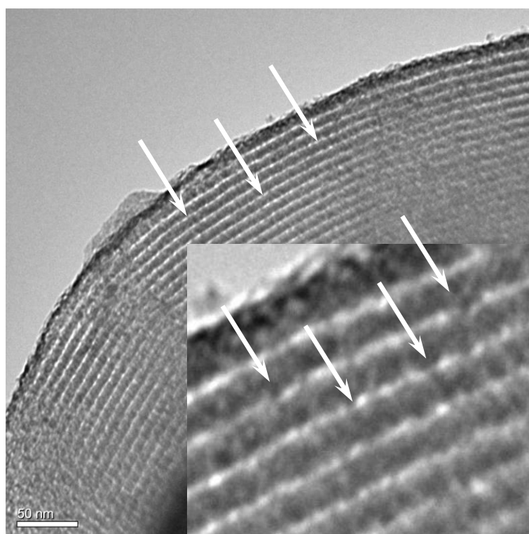
SI Figure 1 TEM image of CMK-3-1.
