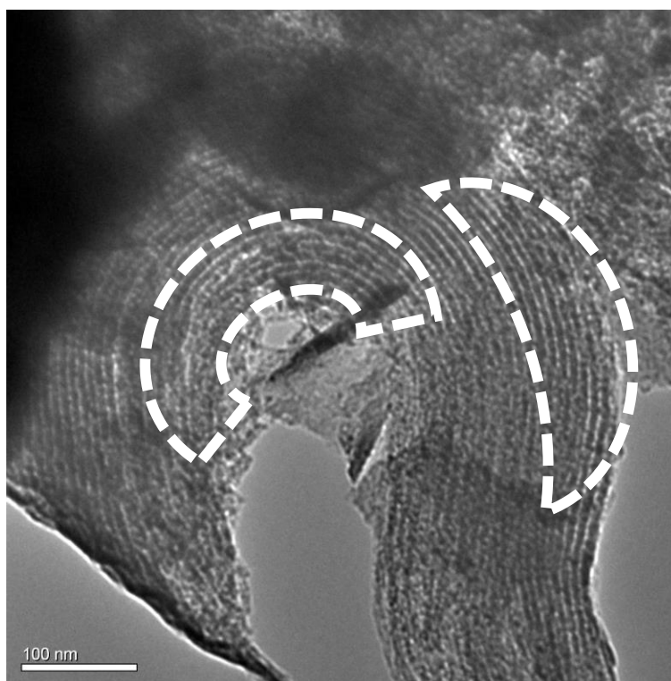
SI Figure 2 TEM image of CMK-3-2.
