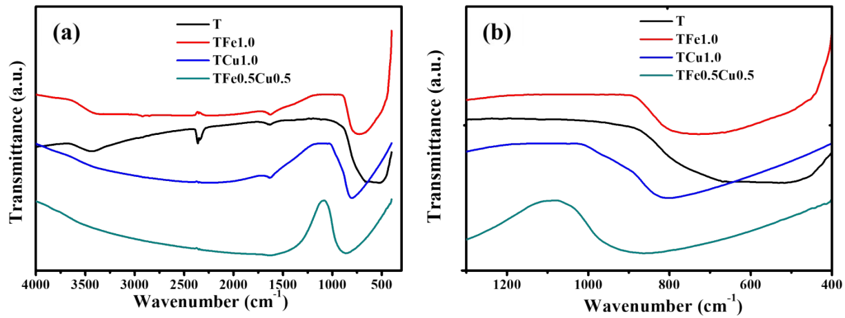
Figure S2: FTIR spectra (a) whole, and (b) finger print region of \text{TiO}_2 , \text{TFe}_{1.0} , \text{TCu}_{1.0} and \text{TFe}_{0.5}\text{Cu}_{0.5}
