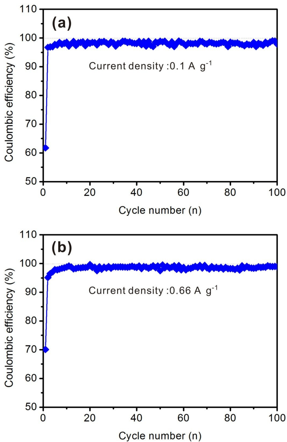
Figure S1. Coulombic efficiencies of the Sb/CCNFs composite at 0.1 A g -1 (a) and 0.66 A g -1 at different cycles.
