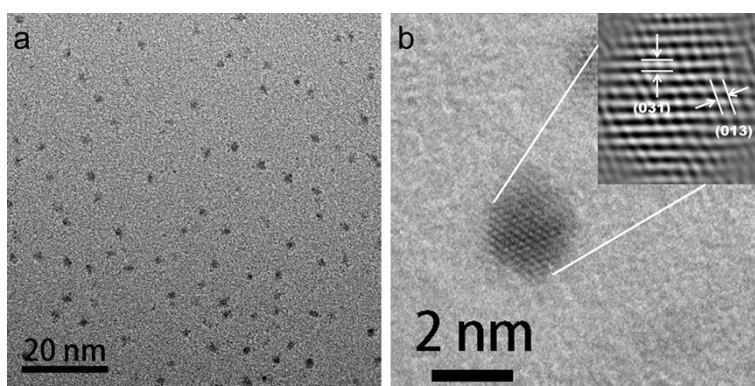
Figure S1. The TEM image (a) and HRTEM image (b) of the Ag 2 Se QDs.
