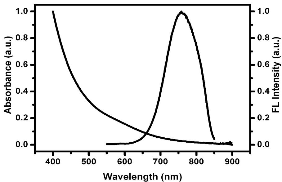
Figure S3. The NIR PL emission spectrum and optical absorption spectrum of \text{Ag}_2\text{Se} QDs.
