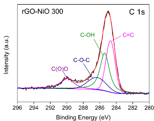
Figure S1 High resolution XPS of C 1s of rGO-NiO 300
