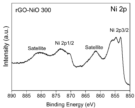
Figure S3 High resolution XPS of Ni 2p of rGO-NiO 300
