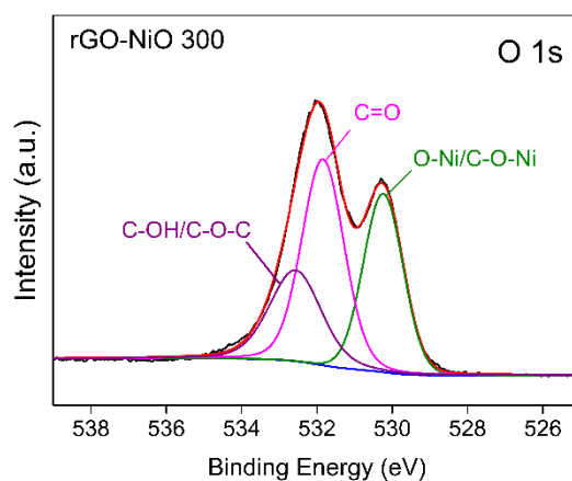
Figure S2 High resolution XPS of O 1s of rGO-NiO 300
