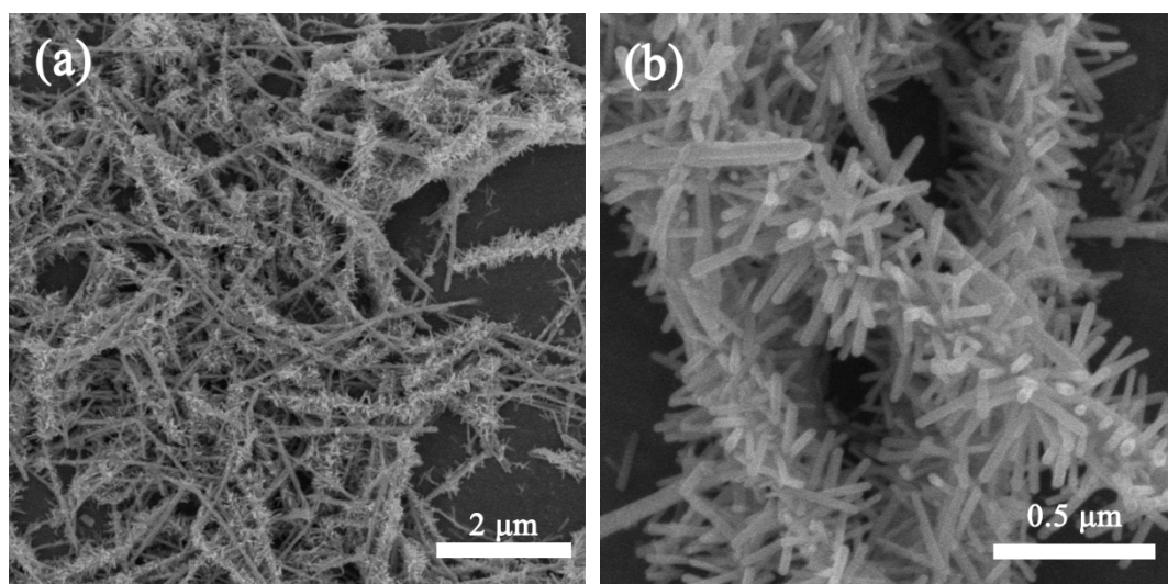
Figure S1. (a) Low and (b) high magnification FESEM images of the Ag@ZnO nanowires.
