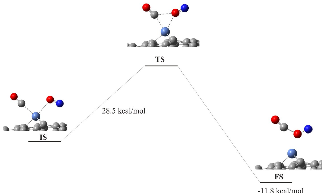
Figure S1. Reaction pathway related to the of CO + NO reaction over Ni-graphene
