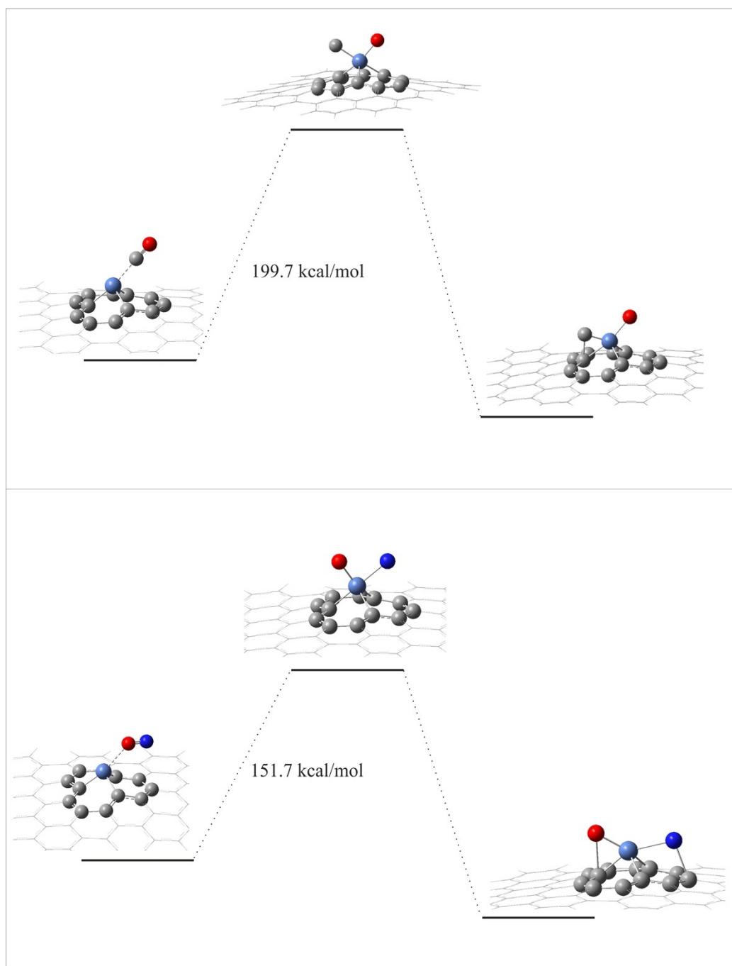
Figure S2. Reaction pathways of CO and NO decomposition over Ni-graphene
