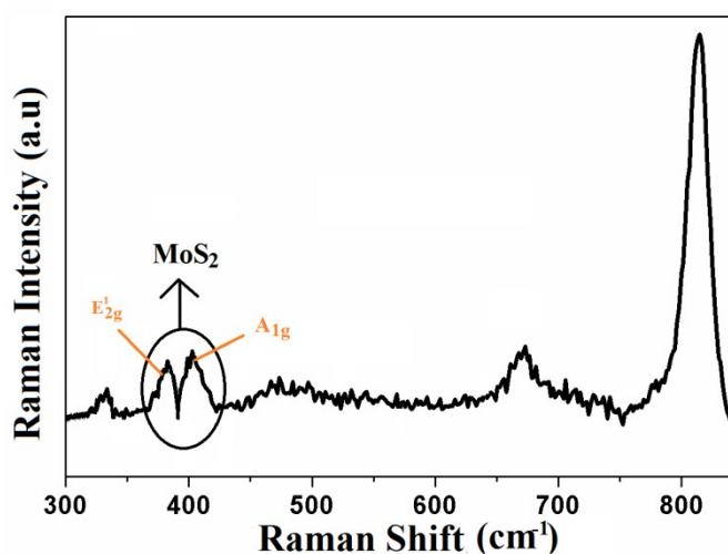
Fig. S1 Raman spectrum of the MSW2.0 film
