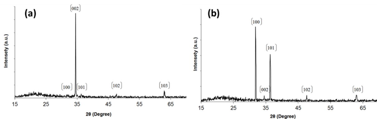
Figure 1. X-ray diffraction spectra of (a) ZnO nanorods and (b) nanosheets.
