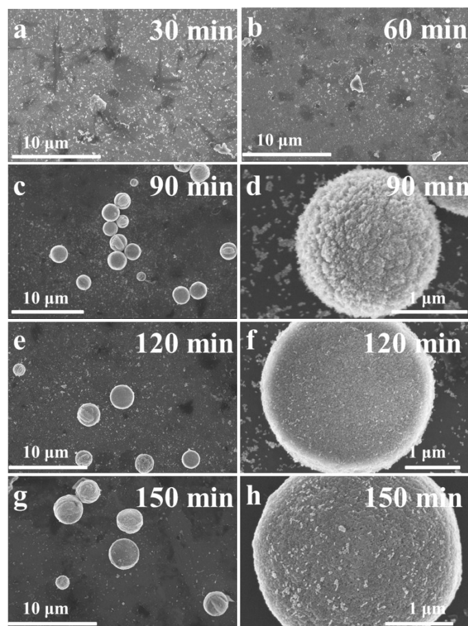
Figure S2. SEM images of AuNR-707/ZnONDK under different reaction time. (a) 30 minutes; (b) 60 minutes; (c, d) 90 minutes; (e, f) 120 minutes; (g, h) 150 minutes. (d), (f) and (h) are magnified images of (c), (e) and (g) correspondingly.
