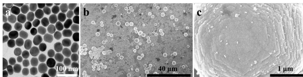
Figure S1. TEM image of AuNSs (a) and SEM images of AuNS/ZnONDK at lower (b) and higher magnification (c).
