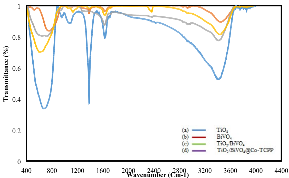
S1. FT-IR spectra of the \text{TiO}_2 and \text{BiVO}_4 nanoparticles, \text{TiO}_2/\text{BiVO}_4 nanocomposite and Co-TPCC@ \text{TiO}_2/\text{BiVO}_4 nanohybrid.
