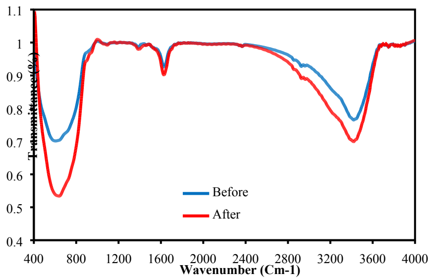
S2. FT-IR spectra of Co-TCPP@TiO 2 /BiVO 4 nanohybrid before and after reuse 8 times.
