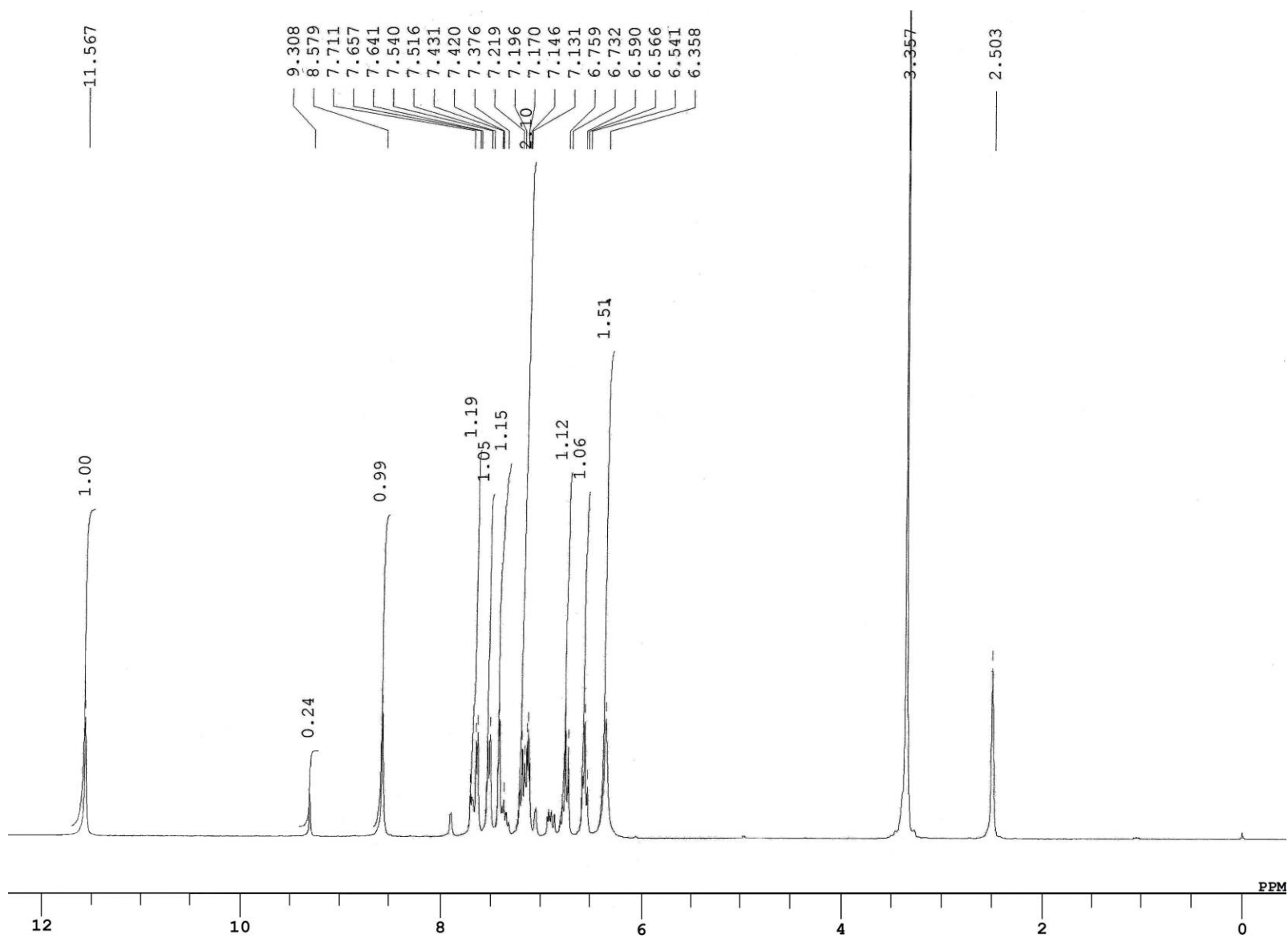
1 H NMR spectrum of ATMBH
