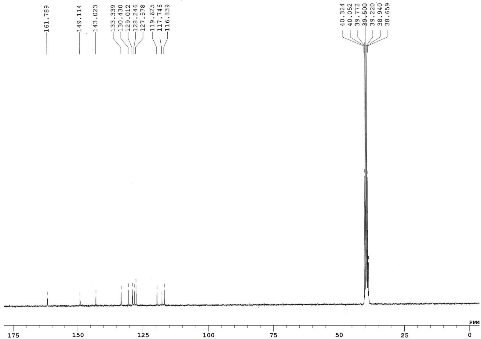
^{13}\text{C} NMR spectrum of ATMBH
