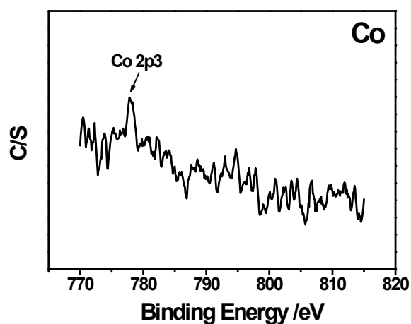
ESI.S2† XPS spectra of SHS: Co 2p region
