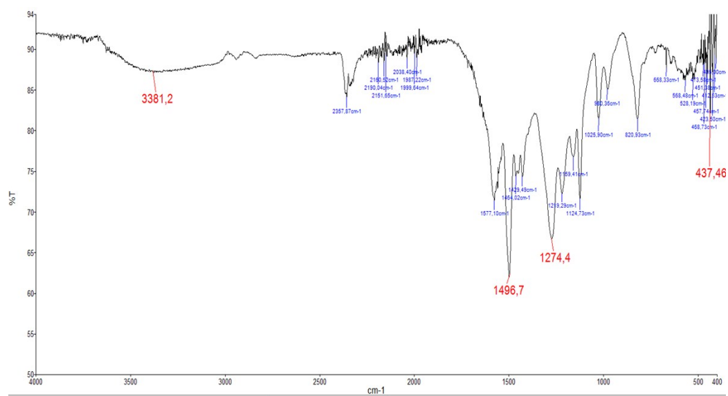
S3. FT-IR spectra for Mn complex
