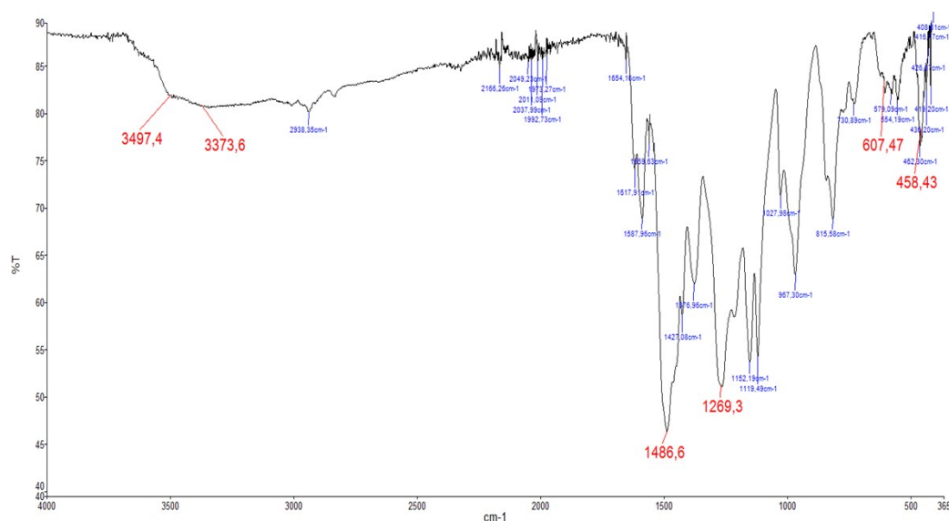
S2. FT-IR spectra for Fe complex
