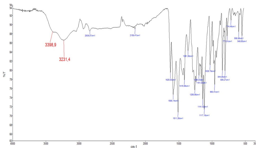
S1. FT-IR spectra for curcumin
