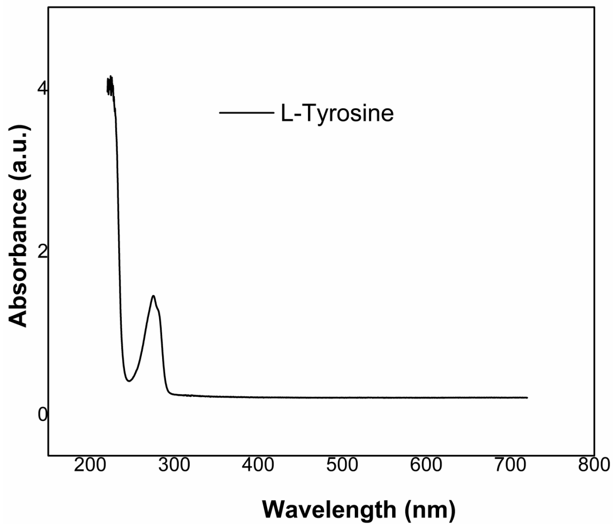
Fig S2: UV-Visible absorption spectra of L-Tyrosine
