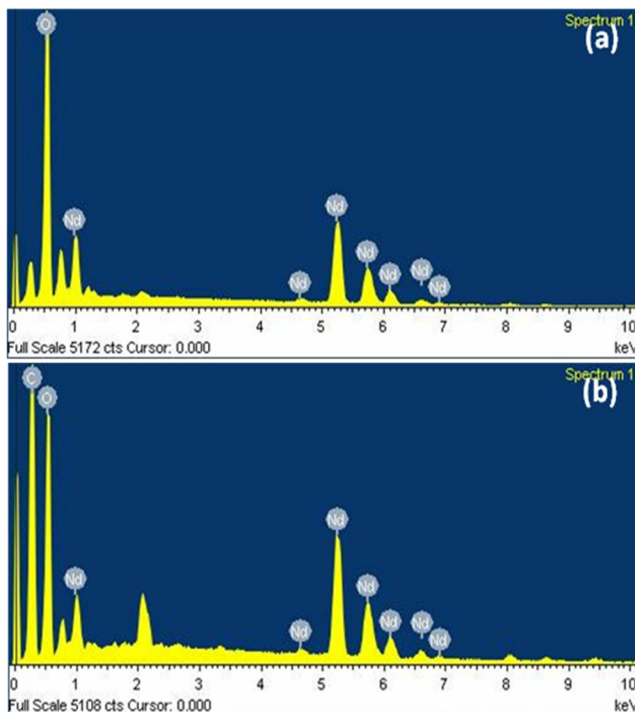
Fig. S1 Energy dispersive X-ray (EDX) spectra of (a) pure \text{Nd}(\text{OH})_3 nanorods and (b) \text{Nd}(\text{OH})_3/\text{G} nanohybrids
