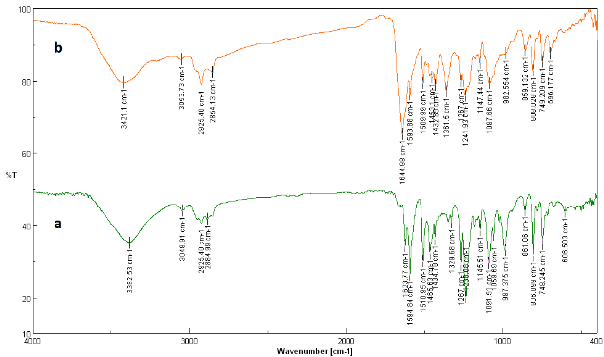
S5. IR spectra of (a) L, (b) L-Fe 3+ complex.
