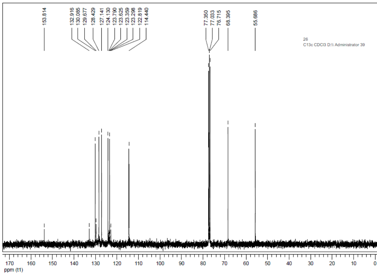
S2. ^{13}\text{C} NMR spectrum of L
