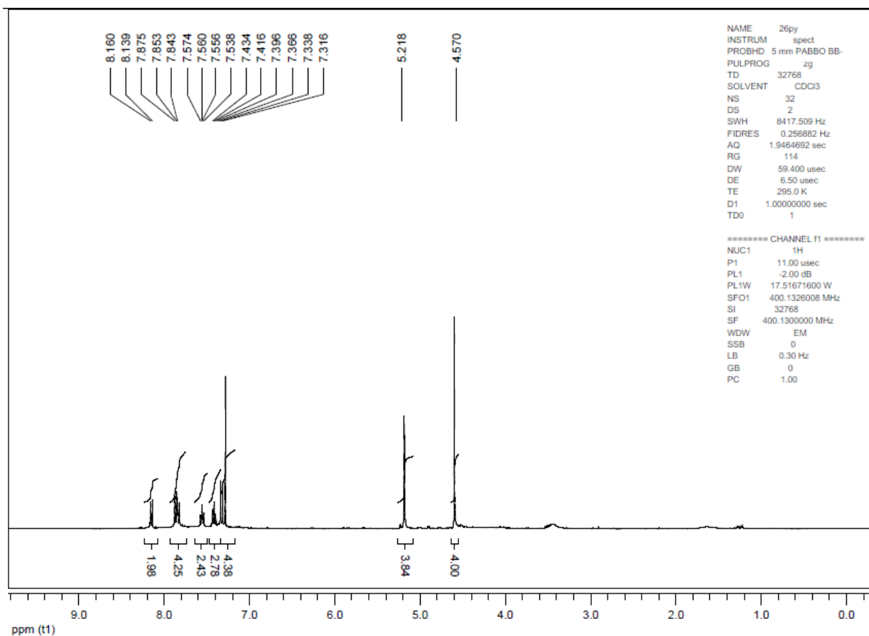
S1. 1 H NMR spectrum of L
