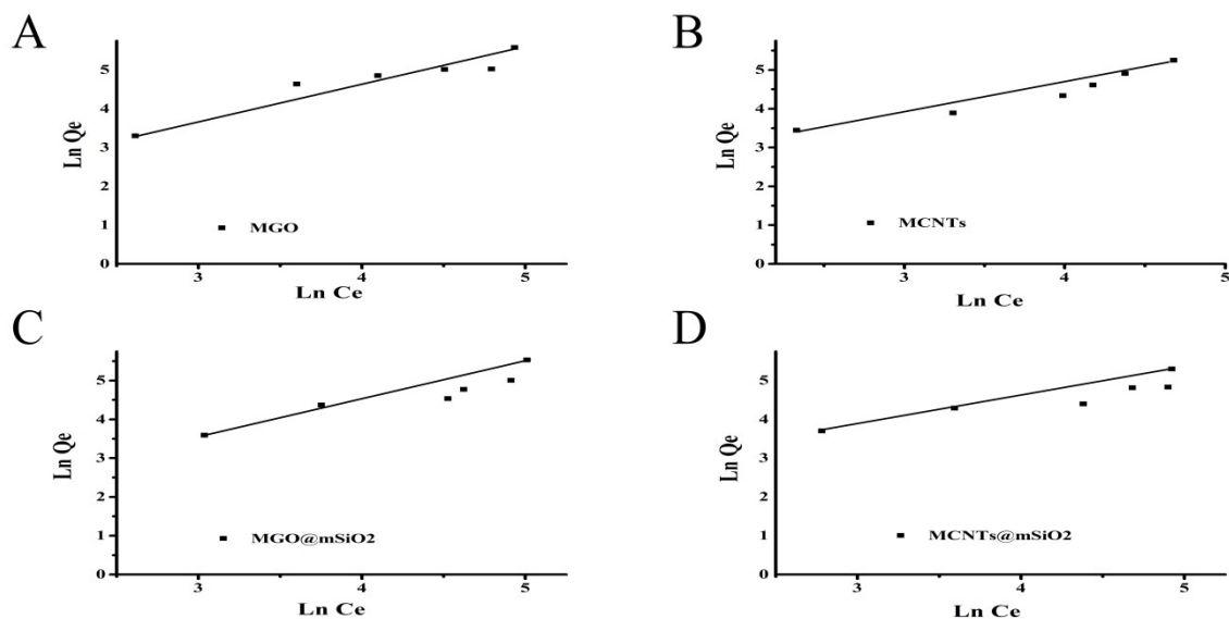
Fig. S1: Freundlich Isotherm model for CPT adsorption onto: A) MGO, B) MCNTs, C) MGO@mSiO 2 , D) MCNTs@mSiO 2 .
