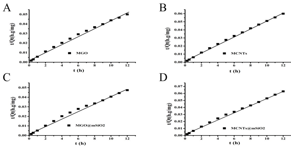
Fig. S3: Pseudo second-order Kinetic plots for CPT adsorption onto: A) MGO, B) MCNTs, C) MGO@mSiO 2 , D) MCNTs@mSiO 2 .
