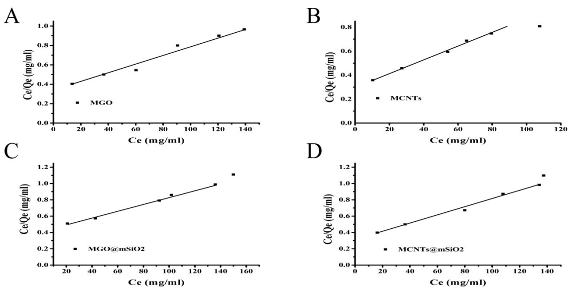
Fig. S2: Langmuir Isotherm model for CPT adsorption onto: A) MGO, B) MCNTs, C) MGO@mSiO 2 , D) MCNTs@mSiO 2 .
