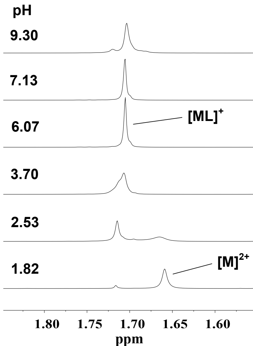
Figure S3. Dependence on pH of the high field region of the NMR spectra registered in the [(\eta^5\text{-Cp}^*)\text{Rh}(\text{H}_2\text{O})_3]^{2+} - \alpha -alaha - system at 298 K; c_{\text{lig.}} = c_{\text{M}} = 10 \text{ mM} ; „M” refers to [(\eta^5\text{-Cp}^*)\text{Rh}]^{2+} .
