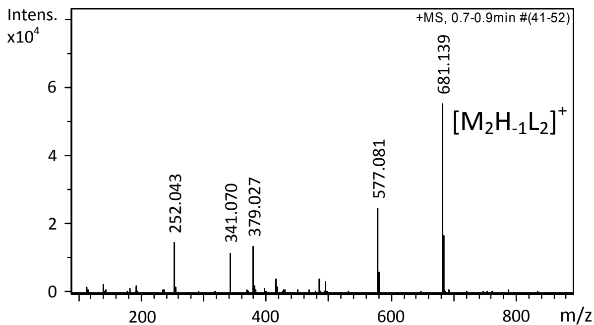
Figure S4. ESI-MS spectrum of the [(\eta^5\text{-Cp}^*)\text{Rh}(\text{H}_2\text{O})_3]^{2+} - \beta -alaha ^- system at 1:2 metal ion to ligand ratio (pH = 10.30); „M” refers to [(\eta^5\text{-Cp}^*)\text{Rh}]^{2+} .
