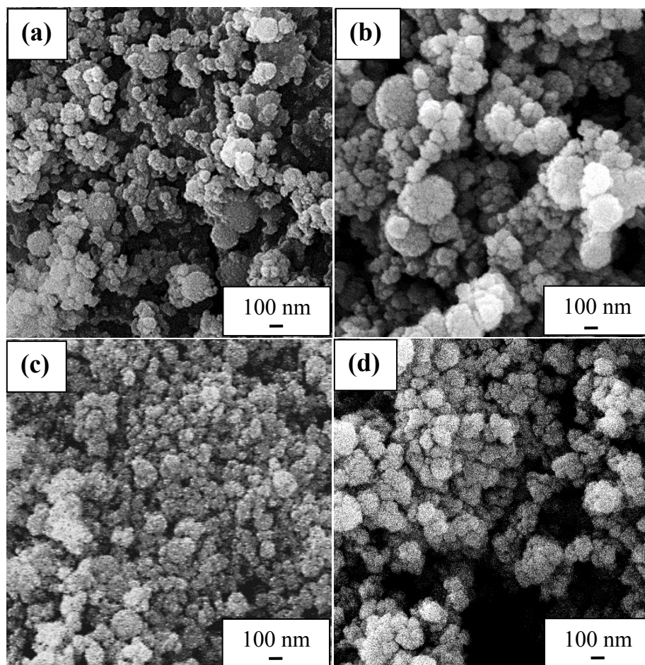
Fig. S1. FE-SEM images of (a) 1%, (b) 2.5%, (c) 5%, and (d) 10% Co-doped Zn(O,S)/Ga 2 O 3 nanocomposites
