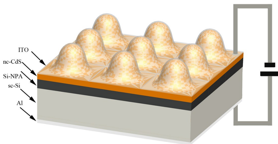
Figure S1 The diagram of final device.
