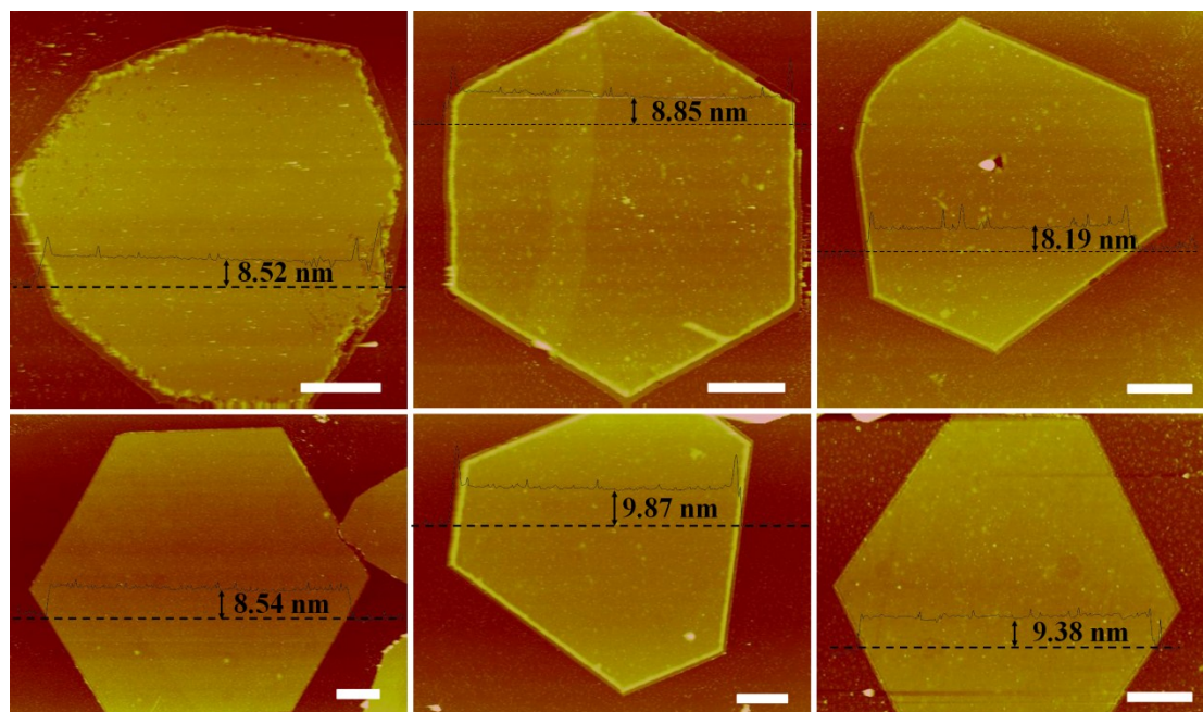
Figure S1. Typical AFM images of the 2D \alpha -Mo 2 C crystals used in this study, showing thickness less than 10 nm. Scale bar: 2 \mu m
