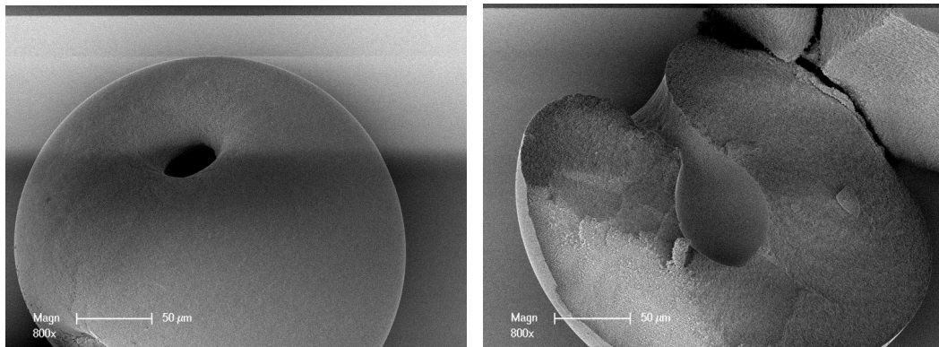
Figure S2 Toroidal assembly from binary mixture of silica nanoparticles of 300 nm and 200 nm at the ratio of 1:1.
