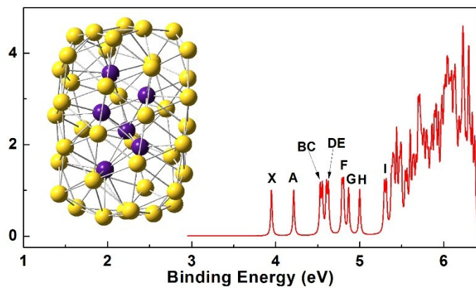
Fig. S3. Anionic Au 6 @Au 42 (C 3 ) and its simulated PES spectrum (peak assignments are tentative).
