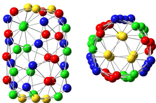
Fig. S1. \text{Au}_{42} ( C_3 ) with color coding to highlight the three distinct helical strands.
