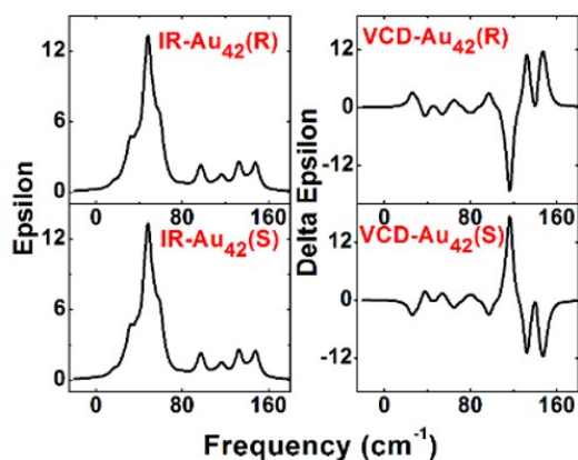
Fig. S2. IR and VCD spectra of \text{Au}_{42} ( C_3 ).
