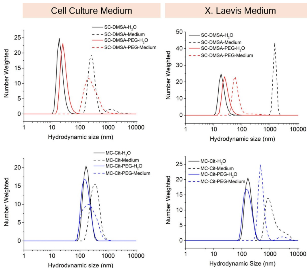
Figure 15. Colloidal properties of nanoparticles suspensions in different biological media.
