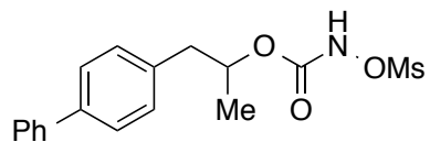
(±)-1-(Biphenyl-4-yl)propan-2-yl N-methylsulfonyloxycarbamate (S33)
