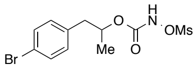
(±)-1-(4-Bromophenyl)propan-2-yl N-methylsulfonyloxycarbamate (S35)
