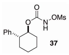
(±)-trans-2-Phenylcyclohexyl N-mesyloxycarbamate (37)
