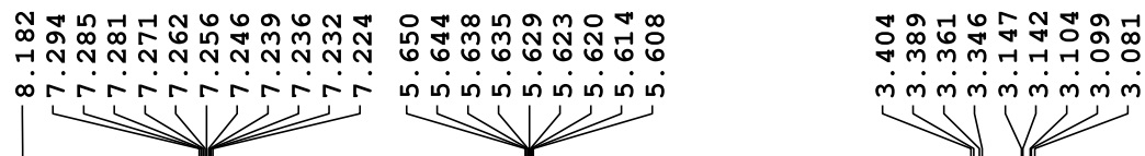
2,3-Dihydro-1H-inden-2-yl N-mesyloxycarbamate (S20)
