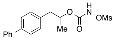
(±)-1-(Biphenyl-4-yl)propan-2-yl N-methylsulfonyloxycarbamate (S33)
