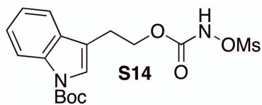
tert-Butyl 3-(2-((mesyloxy) carbamoyl)oxy)ethyl)-1H-indole-1-carboxylate (S14)
