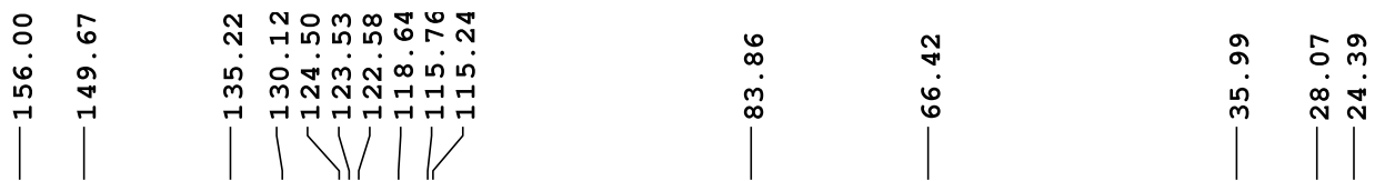
tert-Butyl 3-(2-((mesyloxy) carbamoyl)oxy)ethyl)-1H-indole-1-carboxylate (S14)
