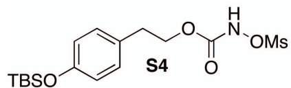
4-((tert-Butyldimethylsilyl)oxy)phenethyl N-mesyloxycarbamate (S4)
