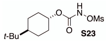
trans-4-(tert-Butyl)cyclohexyl N-mesyloxycarbamate (S23)
