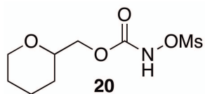
(Tetrahydro-2H-pyran-2-yl)methyl N-mesyloxycarbamate (20)
