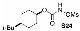
cis-4-(tert-Butyl)cyclohexyl N-mesyloxycarbamate (S24)
