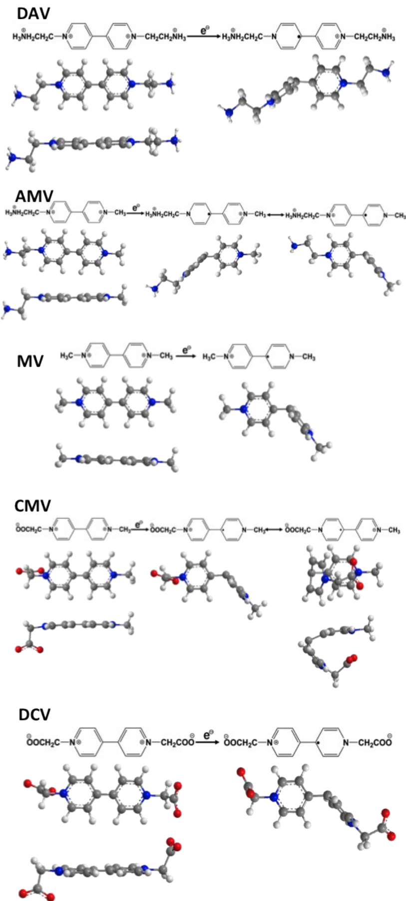
Fig. S1. Conformational Structures of the oxidized and the single-electron reduced form of 4,4'-BPs calculated using MM2.
