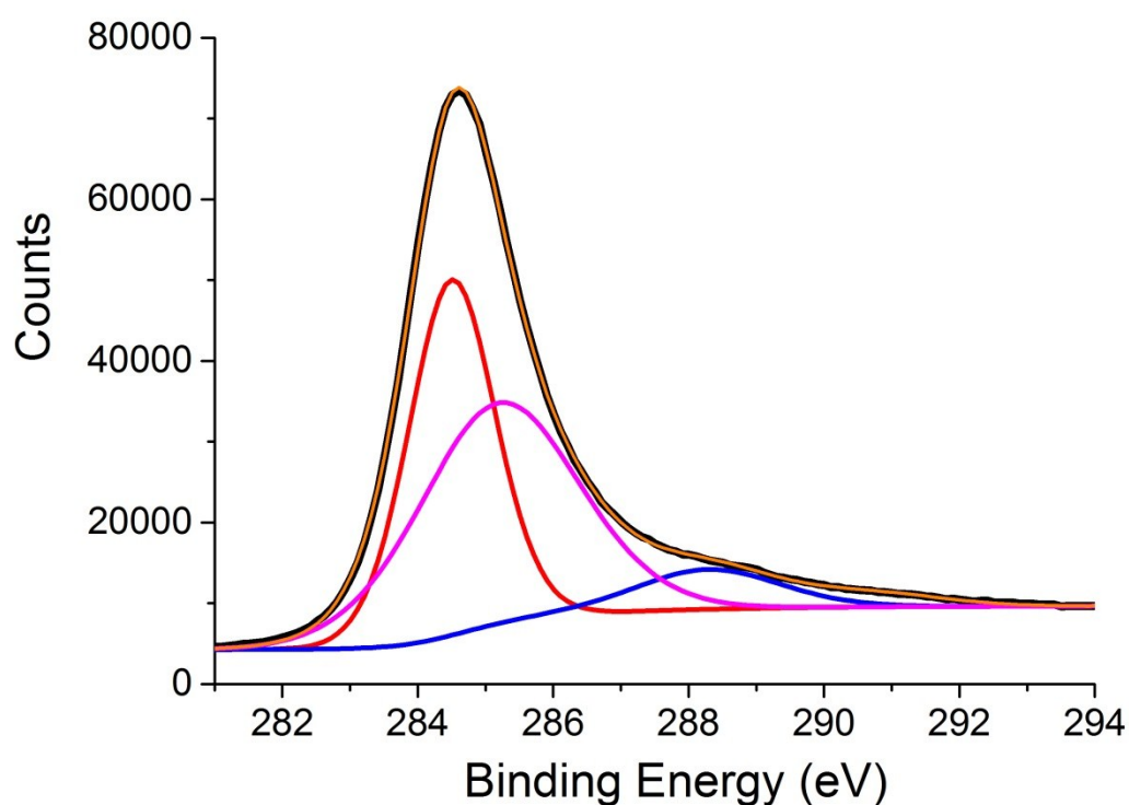
Figure SI1. High resolution XPS peak for C1s recorded for the Cu 2 O/G sample, also showing its best deconvolution into individual components.
